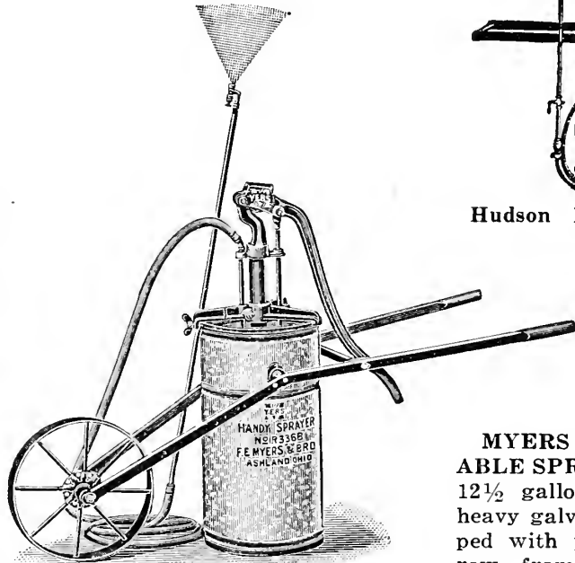
Myers No. R336B Portable
